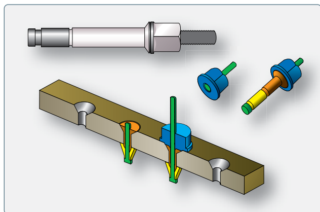
Figure 7-84. Accu-Lok™ installation.
