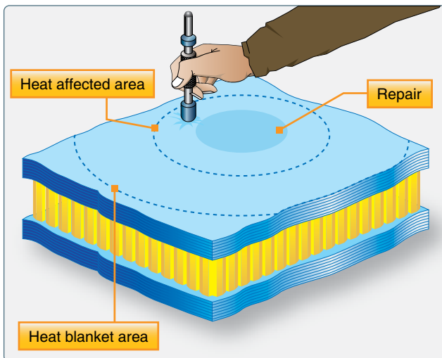
Figure 7-63. Postrepair inspection.
