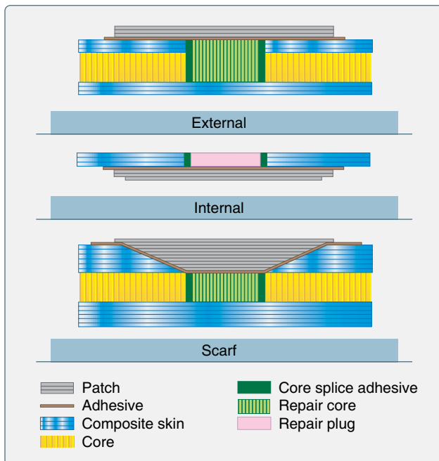
Figure 7-54. Typical repairs for honeycomb sandwich structure.
