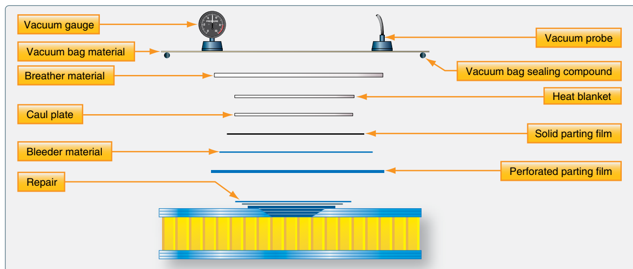
Figure 7-61. Vacuum processing.
