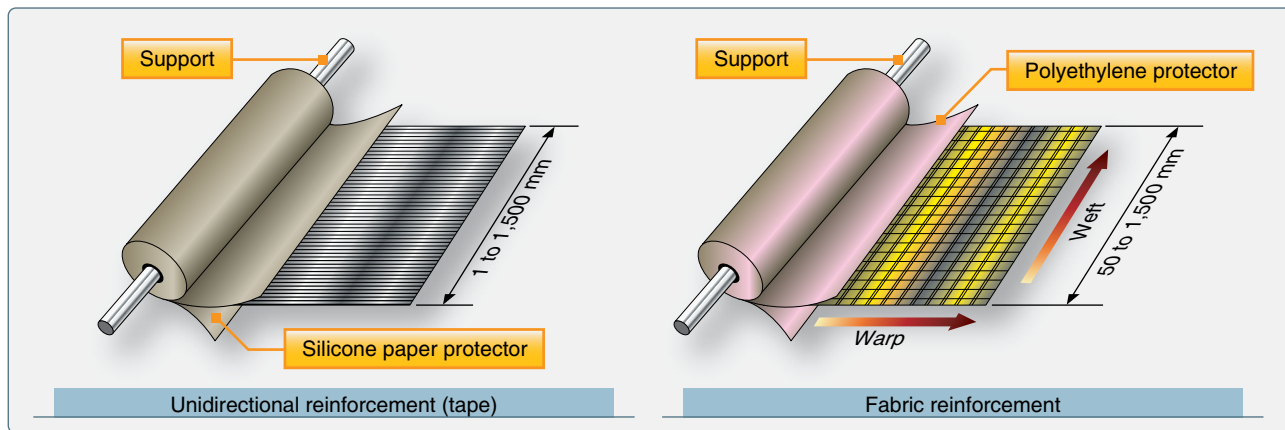
Figure 7-11. Tape and fabric prepreg materials.
