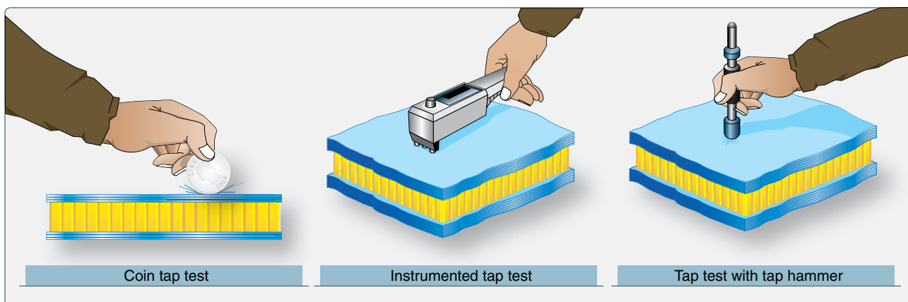
Figure 7-55. Tap testing techniques.
