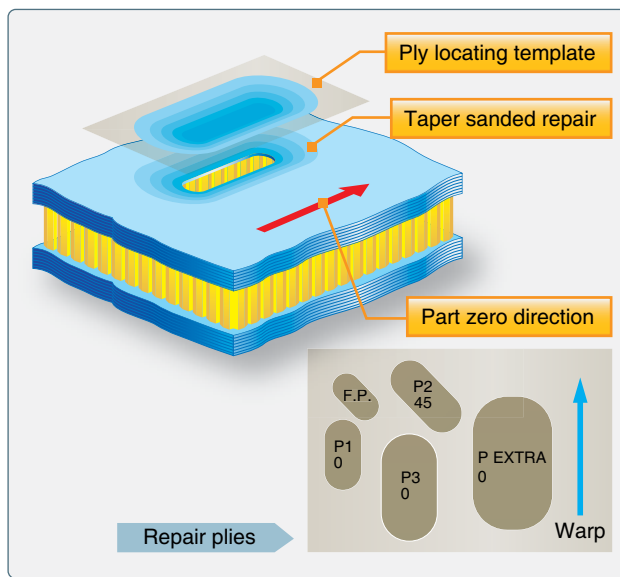
Figure 7-46. Repair layup process.
