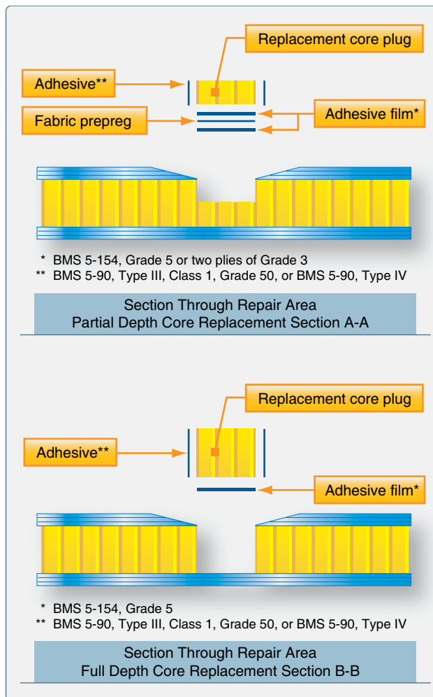
Figure 7-59. Core replacement.
